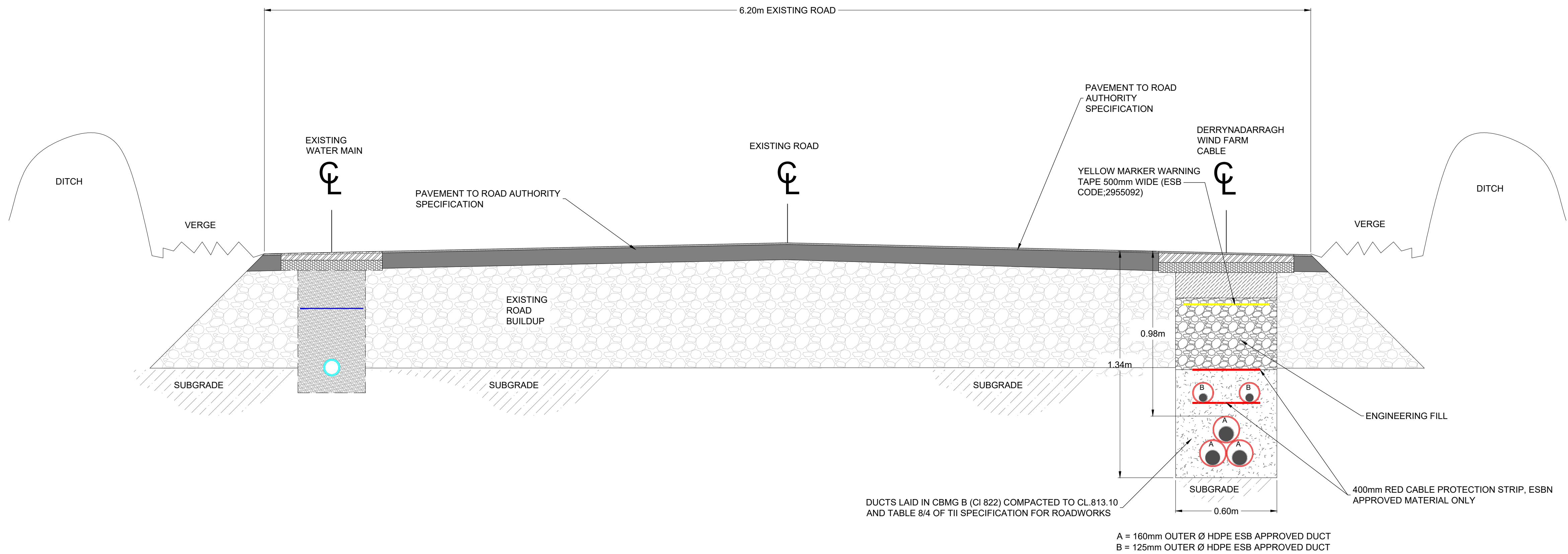
TYPICAL SECTION THROUGH REGIONAL PUBLIC ROAD R420 (SOLID) SCALE 1:15
